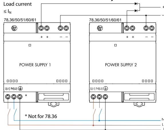
Manual redundancy
