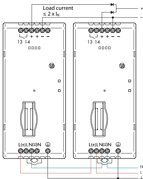
Parallel connection
