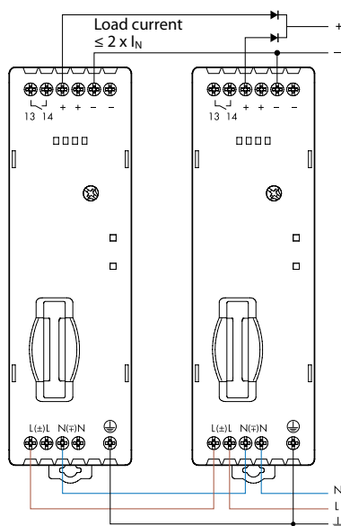
Parallel connection
