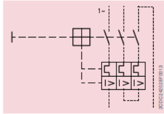
Single-phase operation
