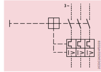
Three-phase operation
