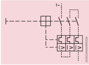
Single-phase operation
